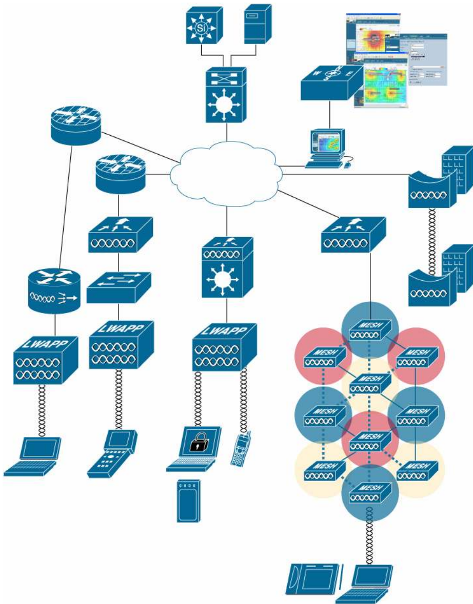
Figure 1. Cisco Unified Wireless Network Elements Work Together to Deliver a Unified Enterprise-Class Wireless Solution
